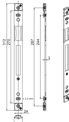
Art. 5303.6
